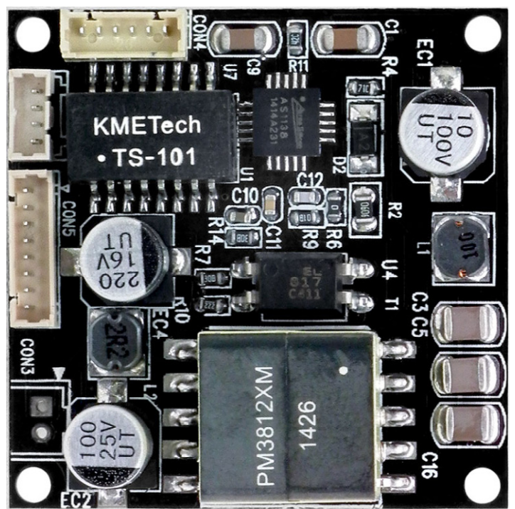
POE BOARD
