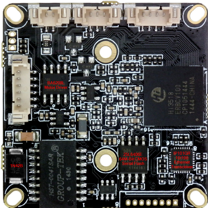
CAMERA BOARD
